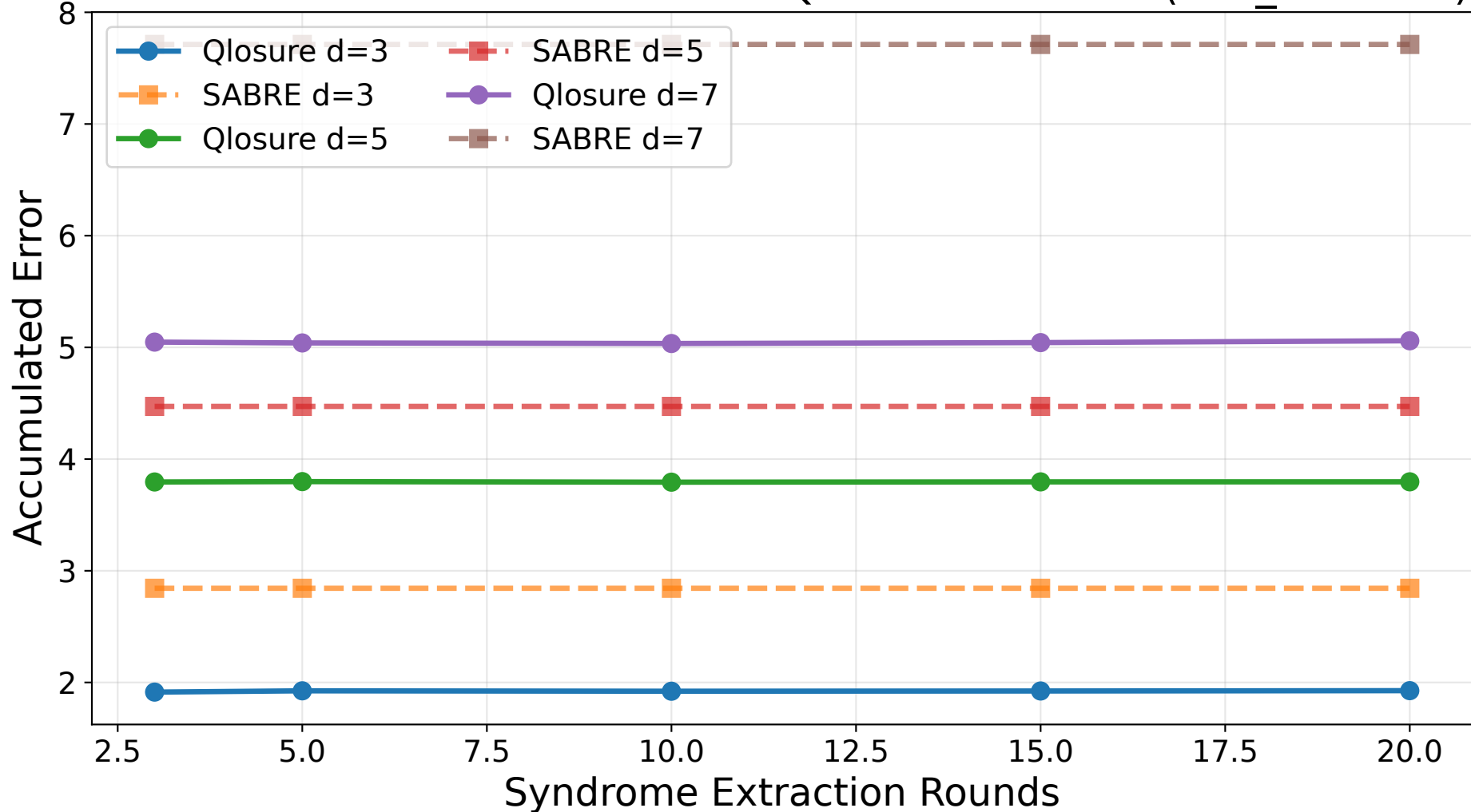
Surface Code Accumulated Error: Qlosure vs SABRE (ibm_brisbane)
