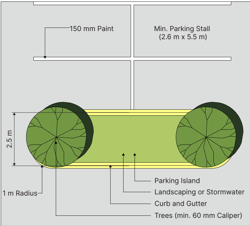
Figure 8.1 Parking Island Requirements
