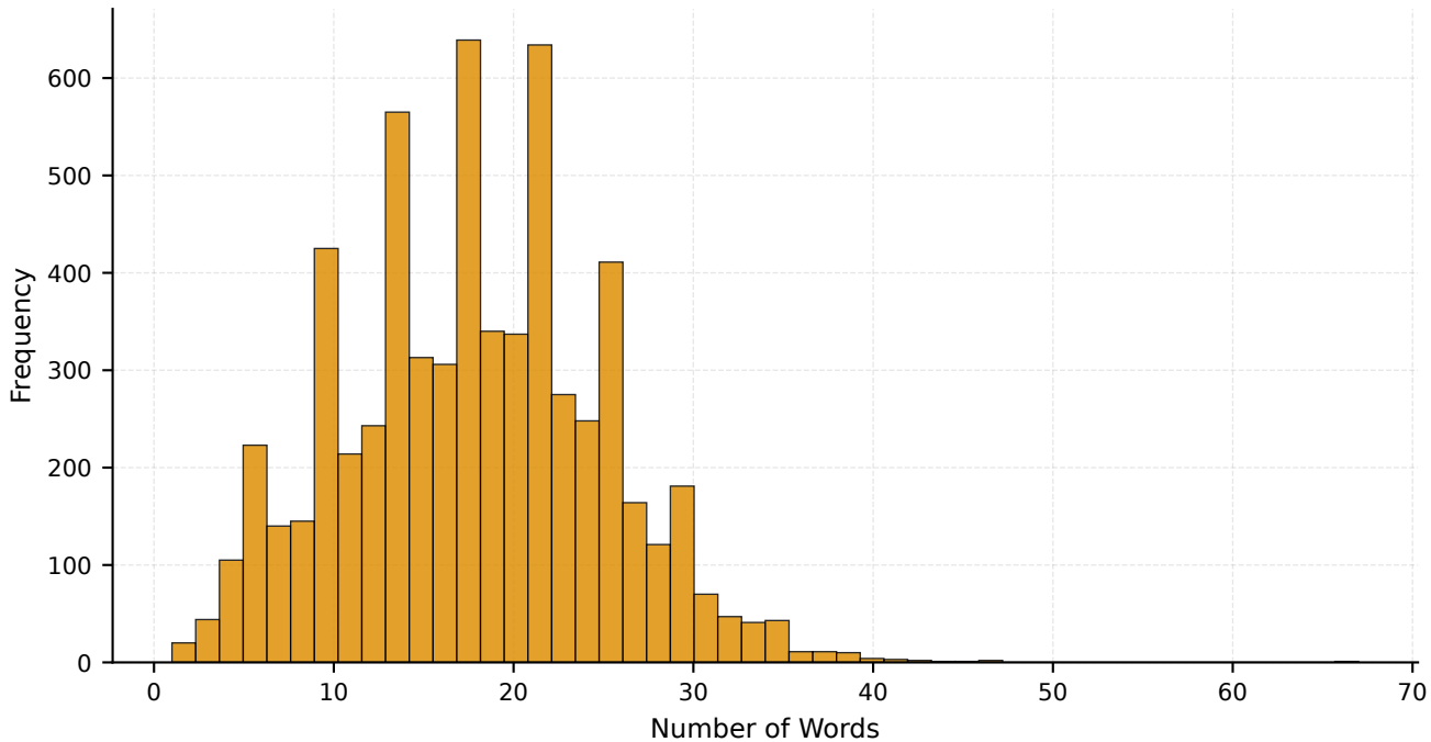
Distribution of Example Length in Words
