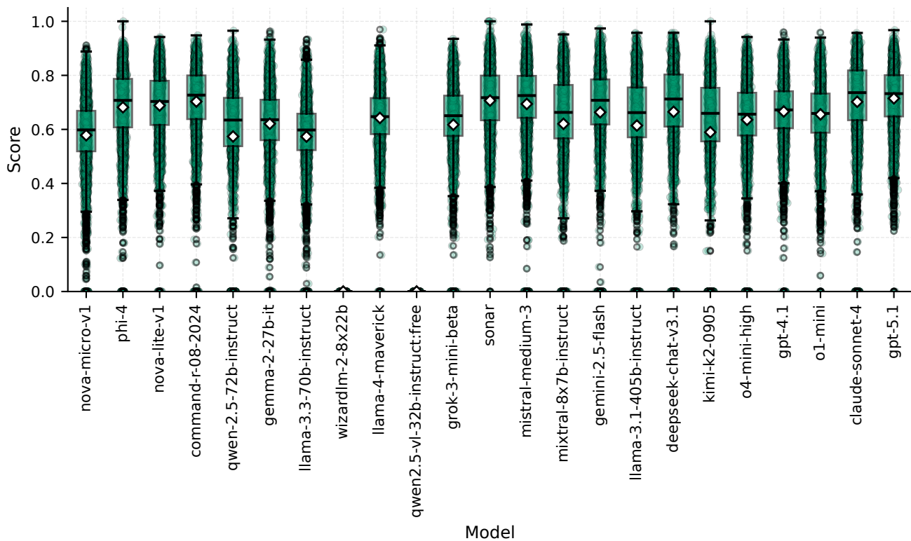
P3: SciBETO-mean
