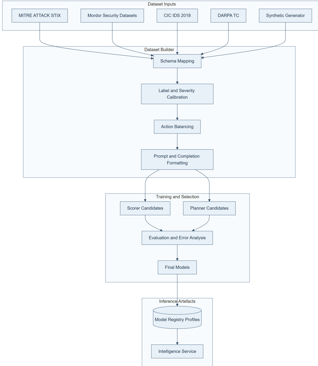
FIGURE 6.1: Dataset construction and training pipeline from public corpora and synthetic generation to deployable scorer/planner model profiles.
