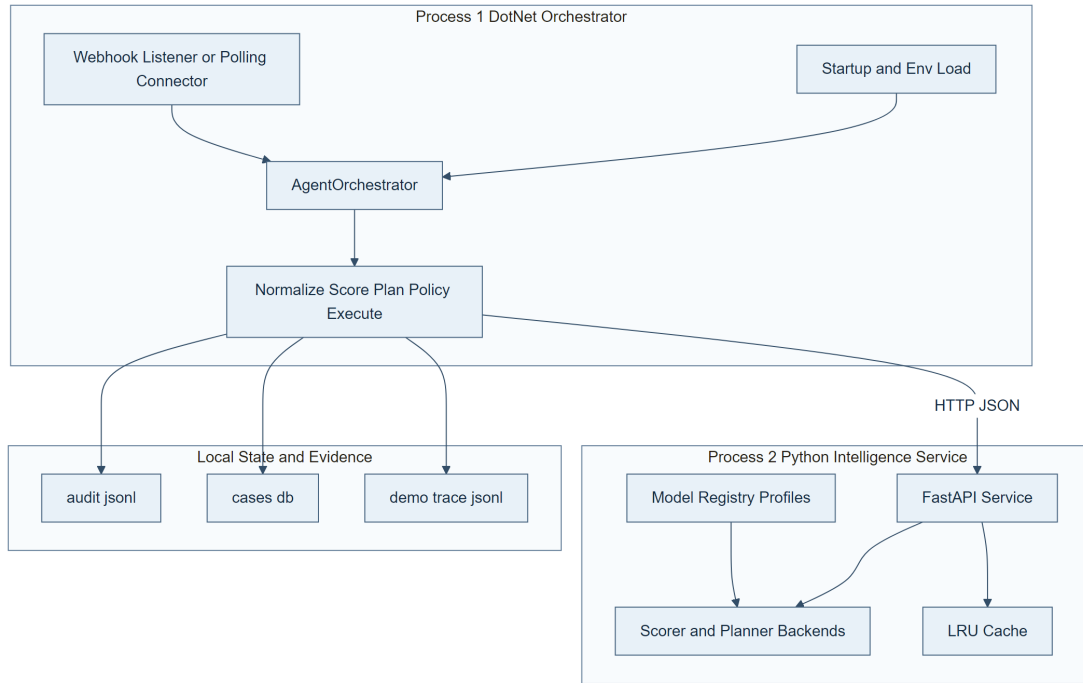
FIGURE 5.1: Implementation runtime boundary: two-process execution model, HTTP contract, and local persistence surfaces.
