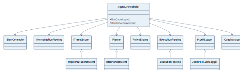
FIGURE 4.3: Core orchestrator class view and its principal collaborators in the C# engine.
