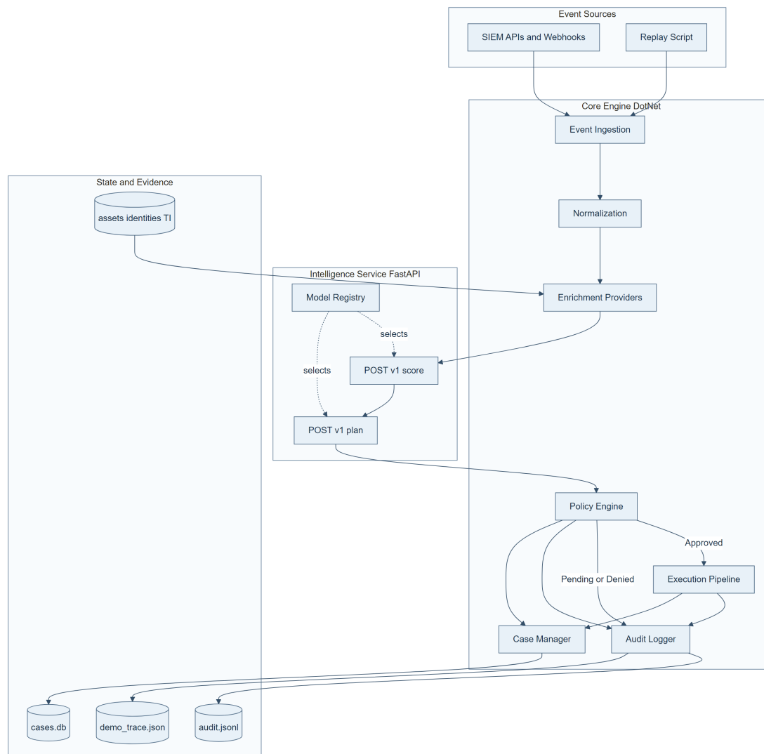
FIGURE 4.4: High-level architecture and control flow across ingestion, intelligence, policy, execution, and evidence layers.
