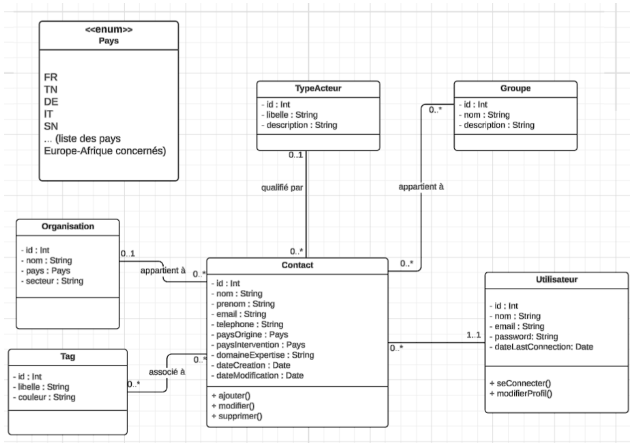
FIGURE 2.2 – Diagramme de classes
