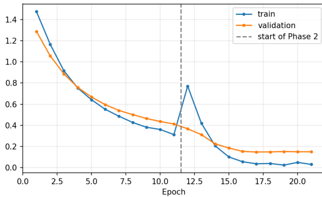
ResNet-50 Loss
