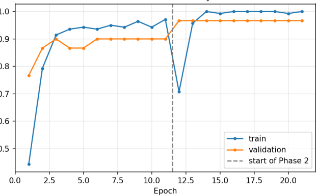
ResNet-50 Accuracy
