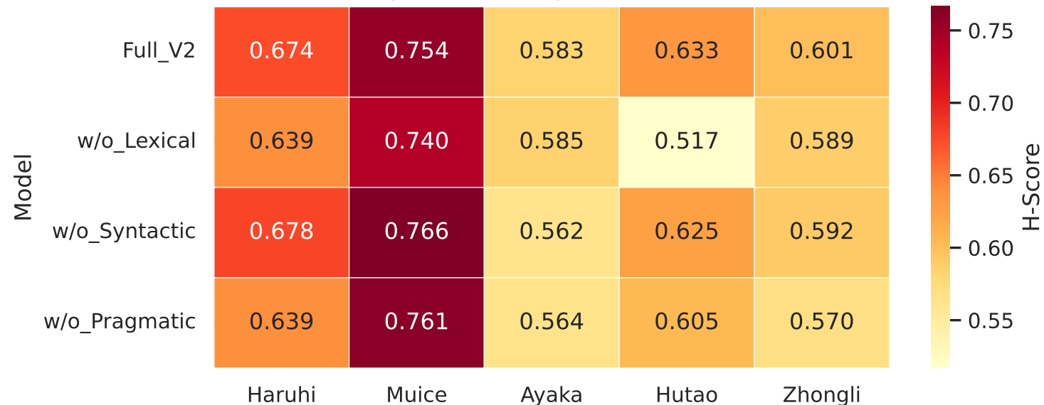
H-Score per Character per Ablation Condition
