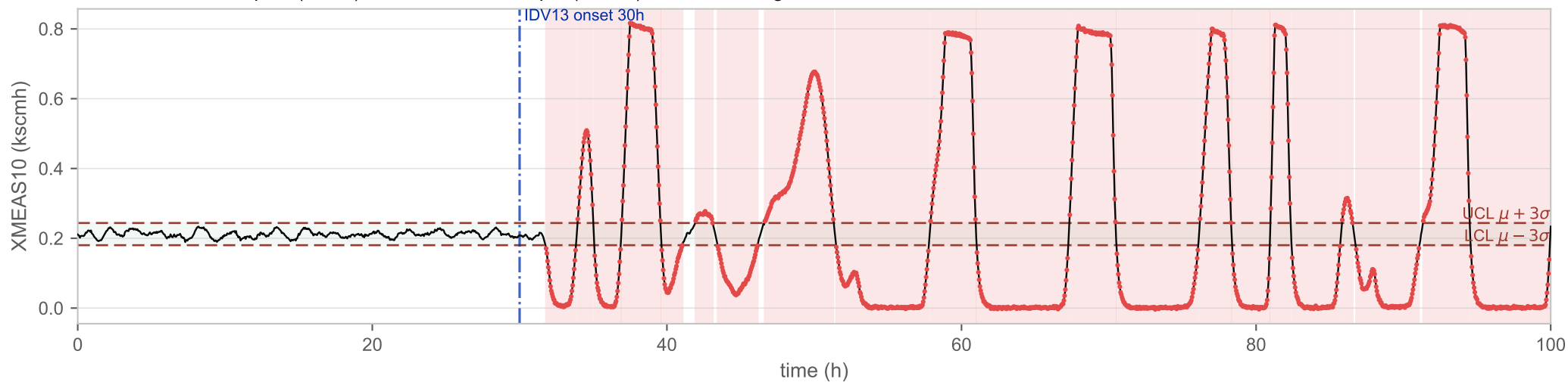
Run10 · 2001 samples (100 h) · out-of-limit 1297 pts (64.8%) · first crossing 31.80 h
