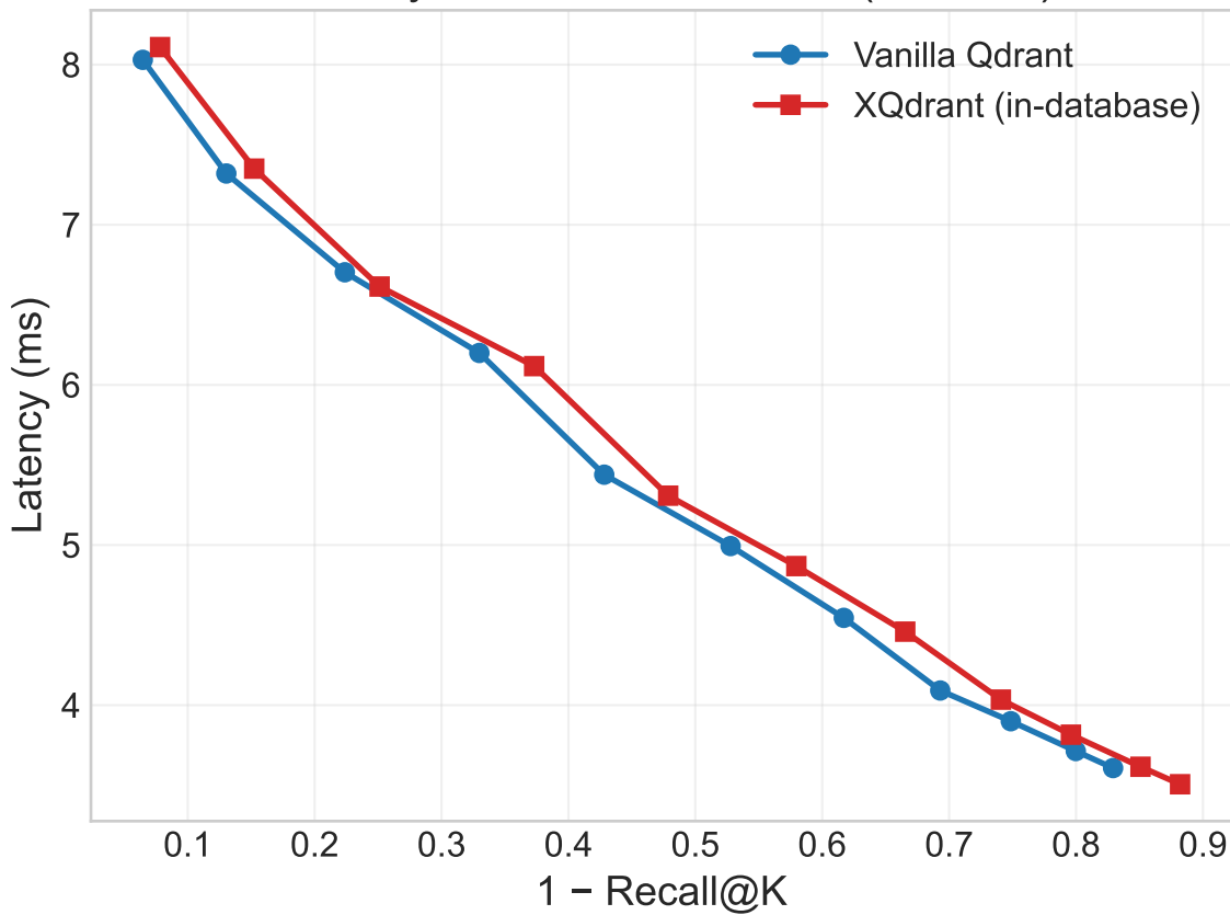
Latency vs. Recall Trade-off (D=1536)
