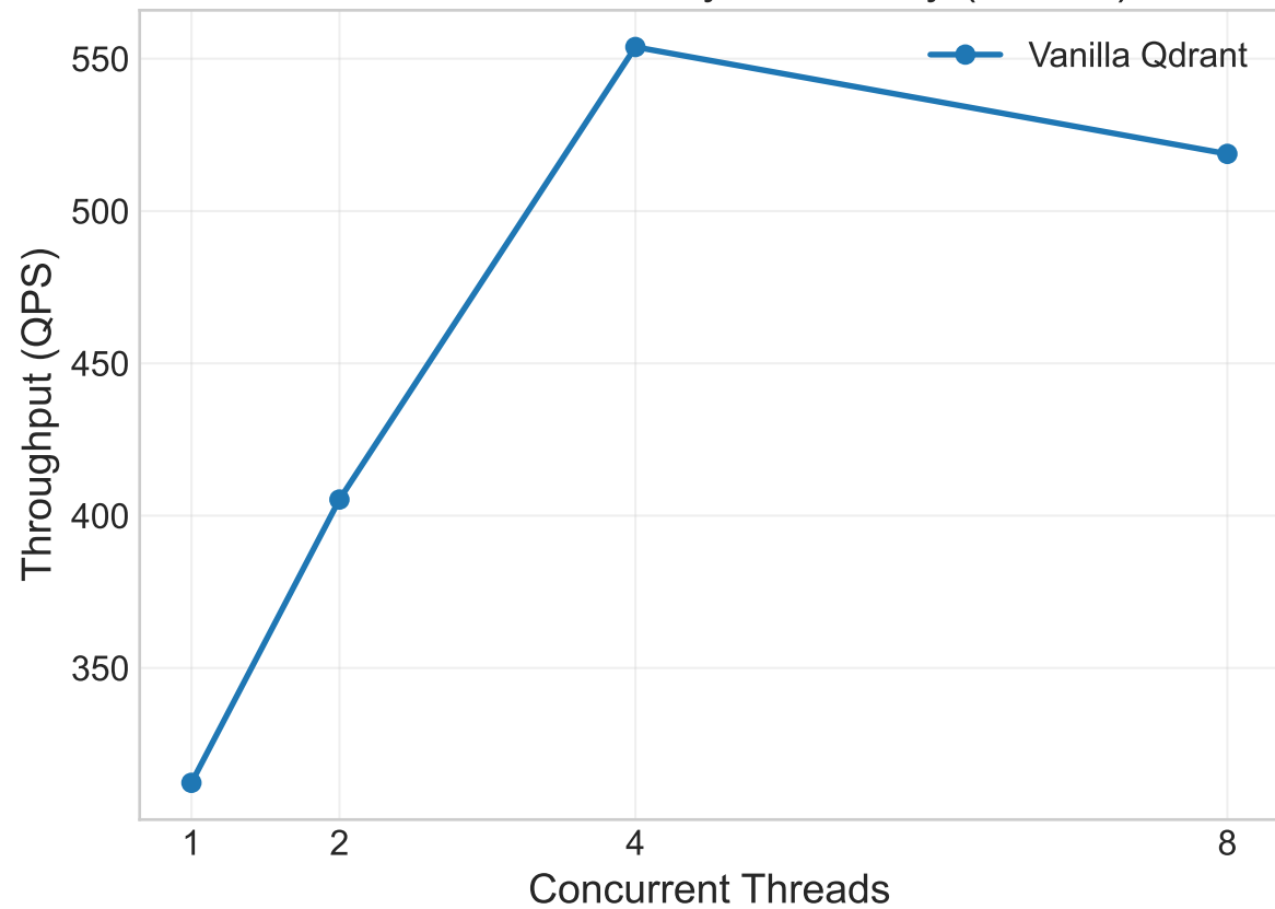
Multi-threaded Query Scalability (D=768)
