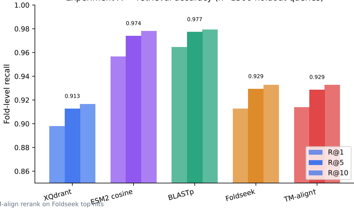
Experiment A — retrieval accuracy (n=1500 holdout queries)
