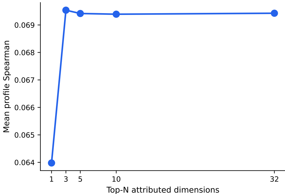
Ablation — attribution dimension count
