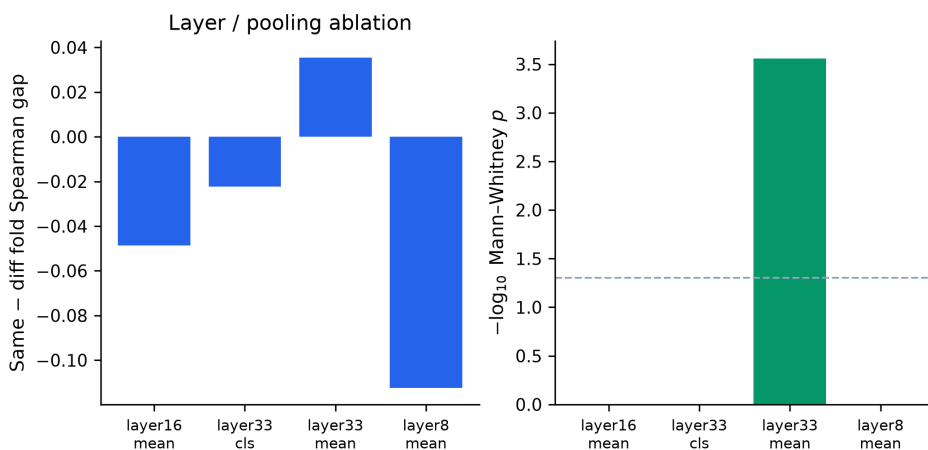
Fig. 12. Layer/pooling ablation: same-fold minus diff-fold Spearman gap. Only last-layer mean pooling is positive.
