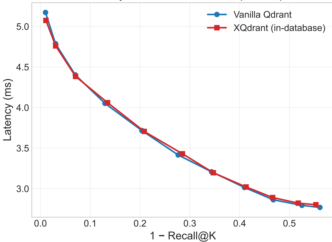
Latency vs. Recall Trade-off (D=768)
