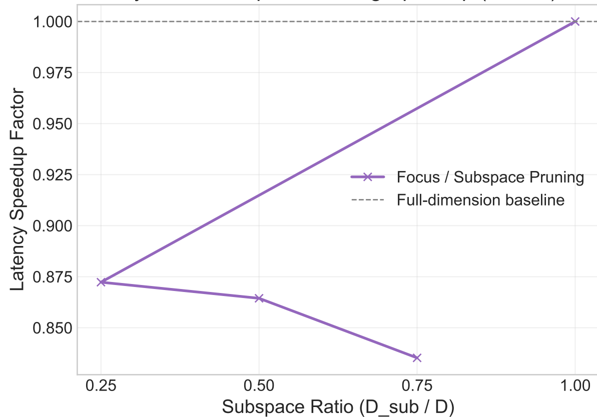
Dynamic Subspace Pruning Speedup (D=768)
