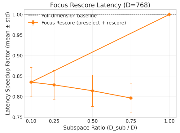
Figure 3: Focus rescoring speedup T_{full}/T_{sub} ( D=768 , host A): values < 1 show rescoring alone does not accelerate search (mean \pm std, T=5 ).
