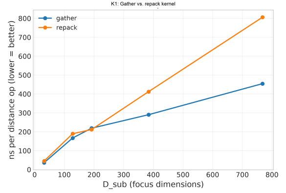
Figure 5: K1: Masked Dot-product kernel cost, repack vs. gather (ns/op, host A).
