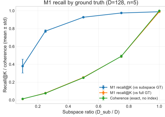
Figure 4: M1 on SIFT1M: Recall@10 against subspace and full-space ground truth, and exact coherence (no index), vs. ratio (mean±std, T=5 ). The full-space curve lies on the coherence curve.
