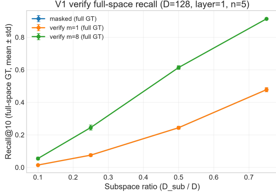
Figure 6: V1 on SIFT1M with L=1 : full-space Recall@10 without verification, with verification at m=1 , and at m=8 (mean \pm std, T=5 ). The unverified curve is hidden under m=1 , which returns the same set by construction.
