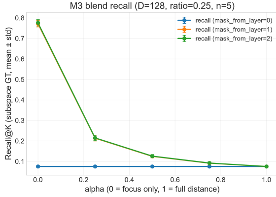
Figure 7: M3 on SIFT1M: subspace Recall@10 vs. \alpha for cut-offs \{0, 1, 2\} at ratio 0.25 (mean \pm std, T=5 ).
