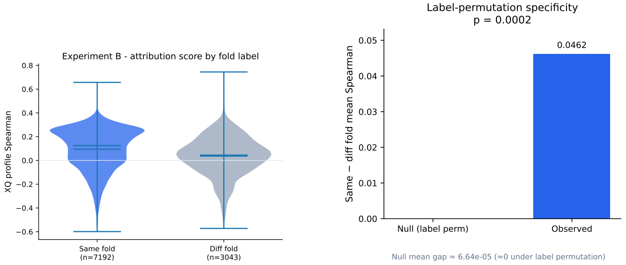
Fig. 3. Experiment B: profile Spearman by fold label (left); label-permutation gap (right).
