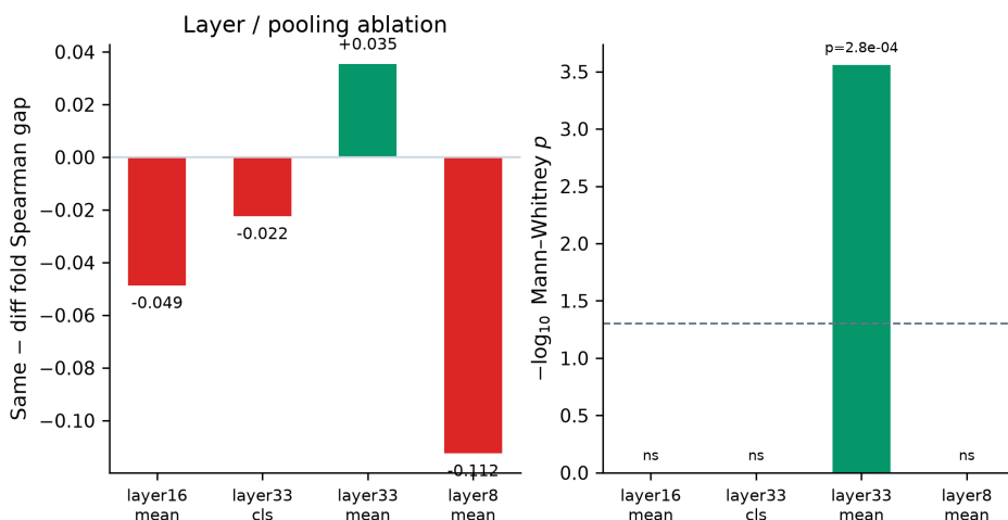
Fig. 12. Layer/pooling ablation: same-fold minus diff-fold Spearman gap. Only last-layer mean pooling is positive.
