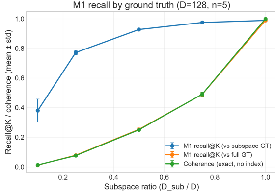
Figure 4: M1 on SIFT1M: Recall@10 against subspace and full-space ground truth, and exact coherence (no index), vs. ratio (mean \pm std, T=5 ). The full-space curve lies on the coherence curve.
