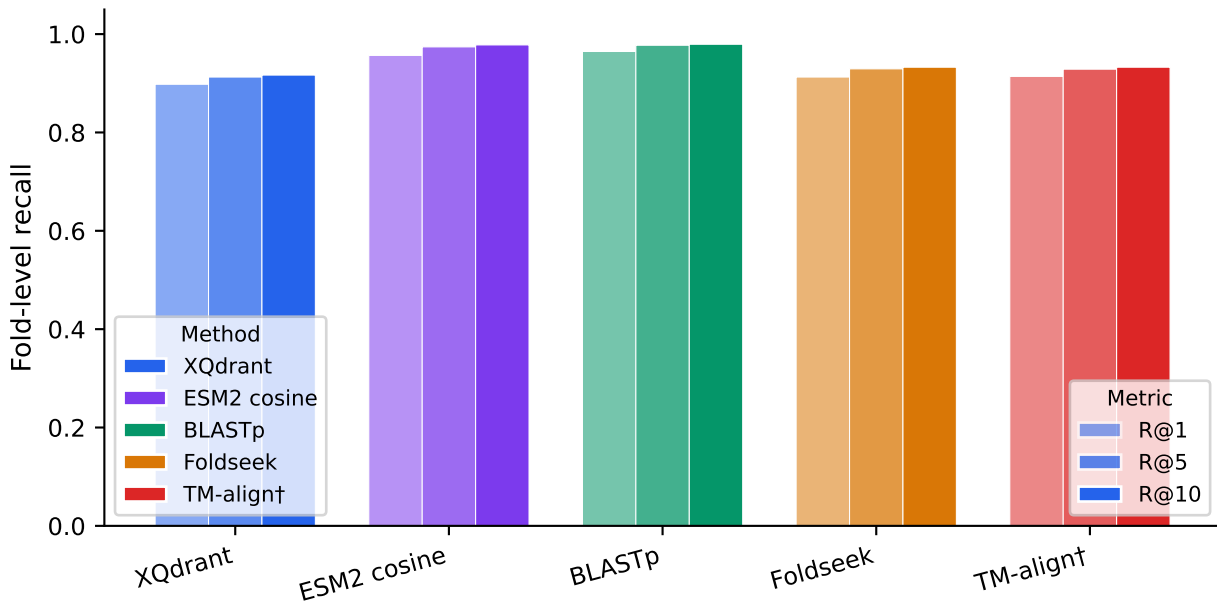
Experiment A - retrieval accuracy (n=1500 holdout queries)
