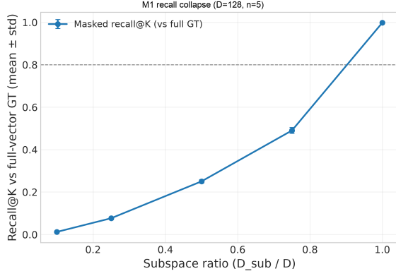
Figure 5: M1 on SIFT1M: Recall@10 vs. full-space ground truth as D_{sub}/D shrinks (mean±std over T=5 trials).
