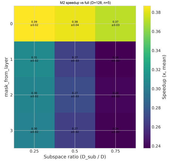
Figure 8: M2 SIFT end-to-end speedup vs. full search: no cell exceeds 1\times , despite recovered recall (mean±std).
