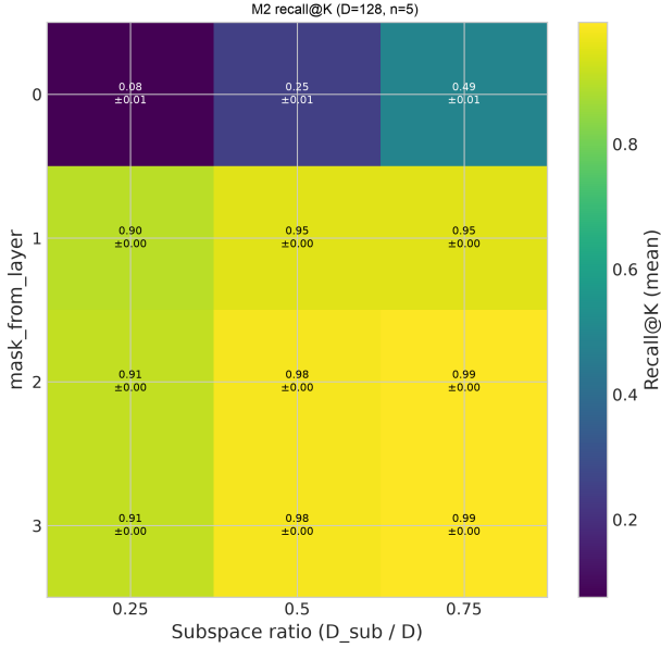
Figure 6: M2 on SIFT1M: recall heatmap over mask\_from\_layer \times subspace\ ratio , gather kernel (cell text: mean±std).
