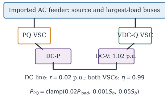
(c) Fully disclosed deterministic AC/DC overlay
