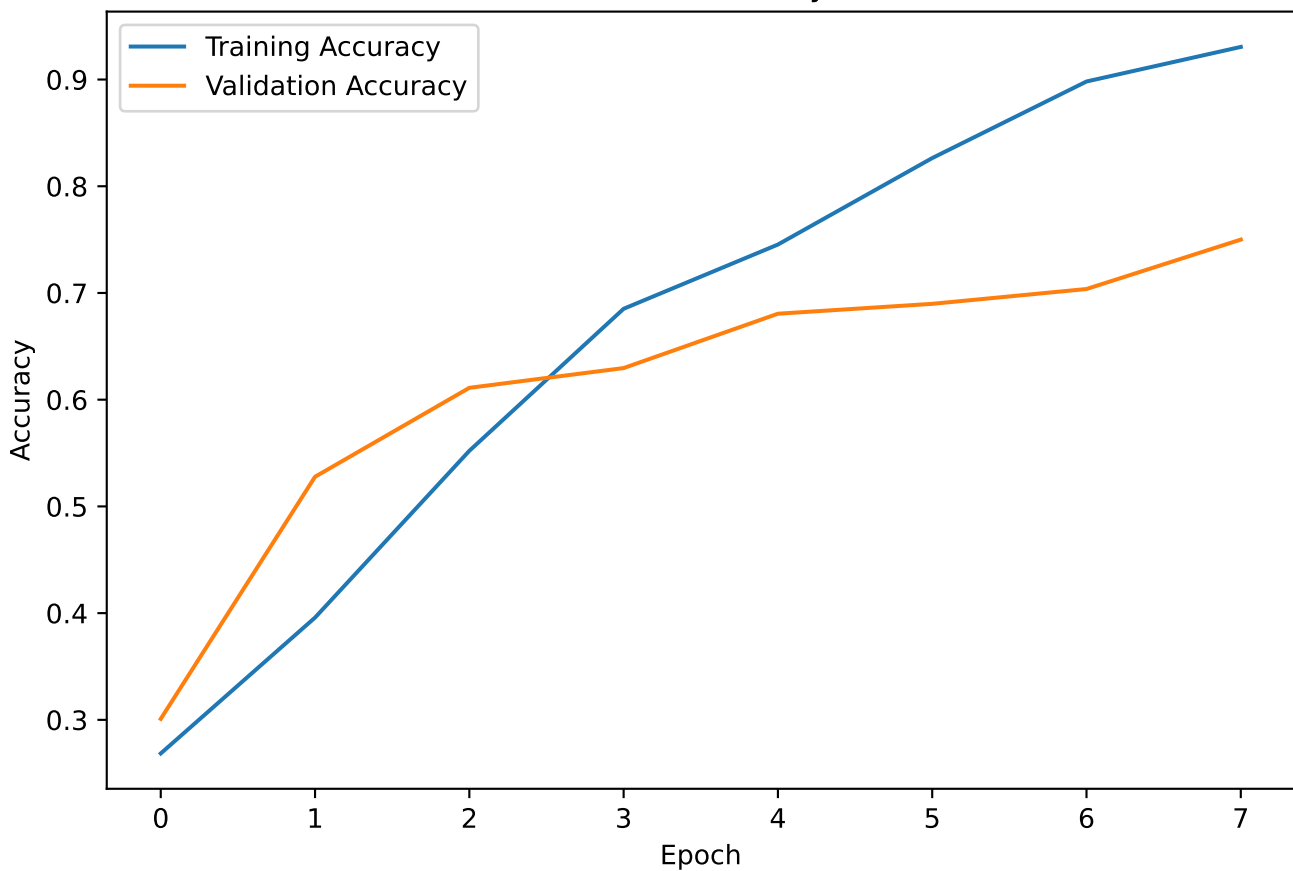
Custom CNN Accuracy Curve
