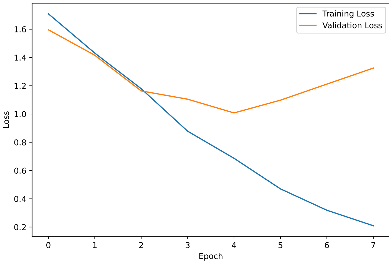
Custom CNN Loss Curve
