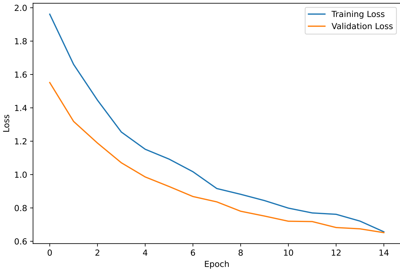
MobileNetV2 Loss Curve
