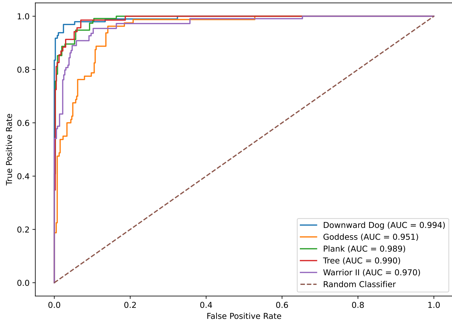
Multi-Class ROC Curves for MobileNetV2
