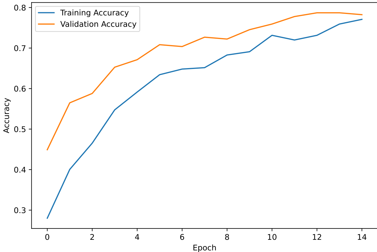
MobileNetV2 Accuracy Curve
