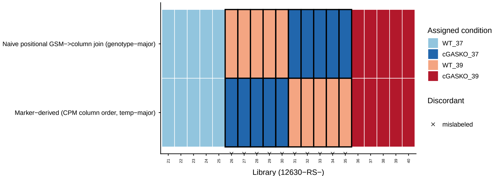
Fig 1d -- Scramble exhibit: positional GSM join mislabels libraries 026–035
