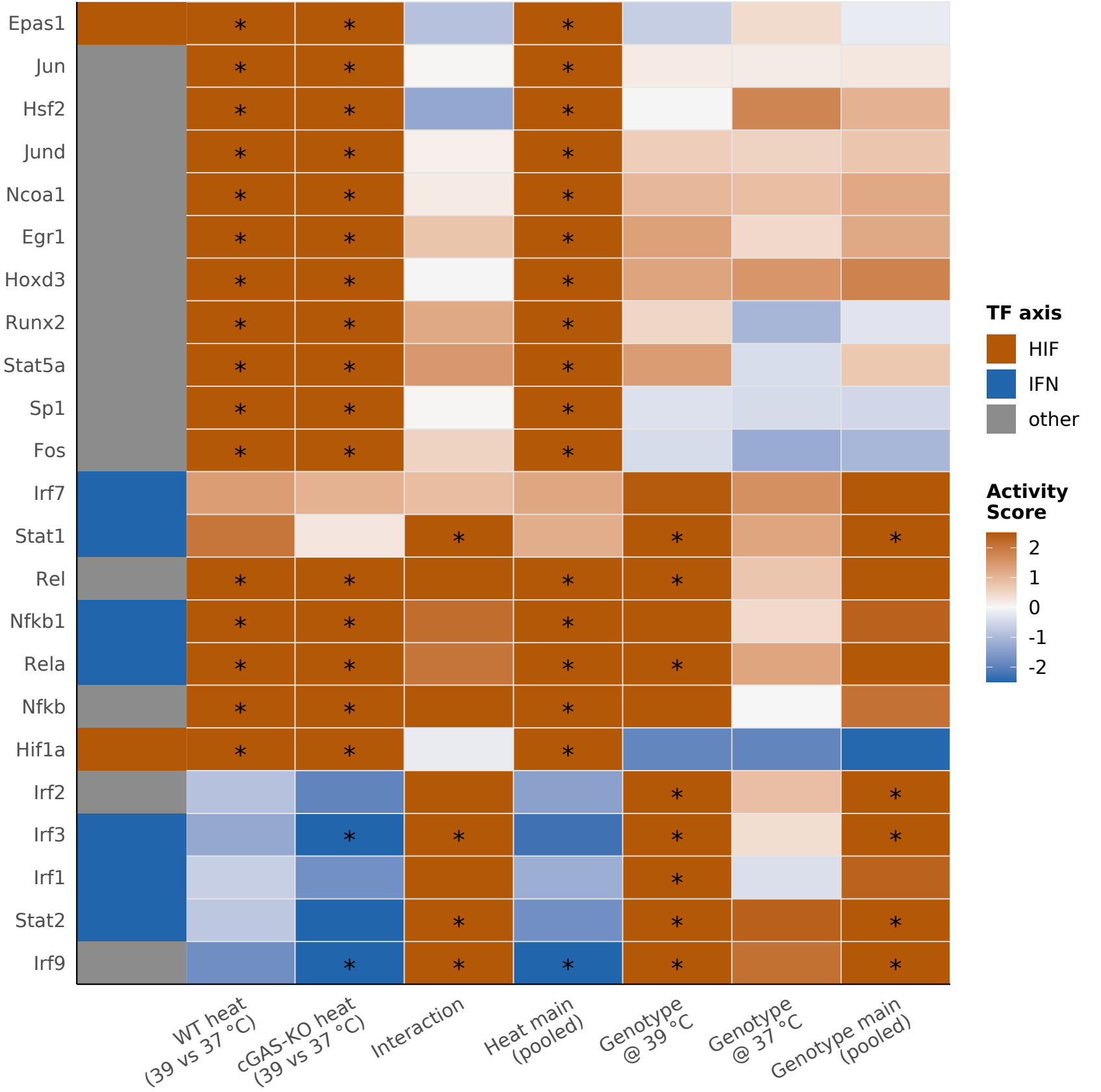
CollectRI TF activity across contrasts (sig in >=2)
