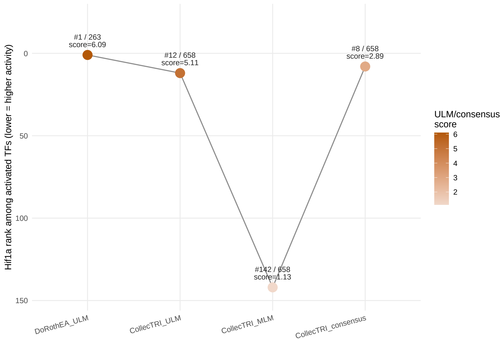
Fig 3c. Hif1a rank cascade across inference method / network (WT_heat)
