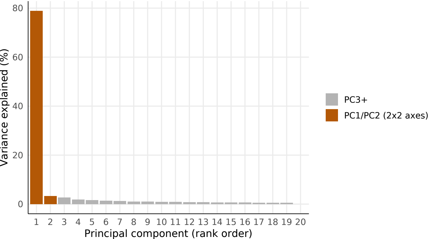
Fig 1c (screen) -- variance explained per PC (top 2000 variable g
