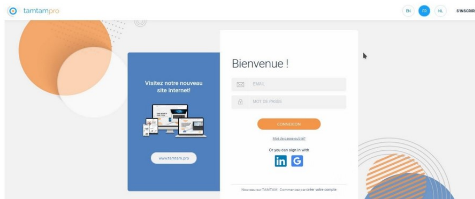
Figure 4.2 – Interface d'authentification
