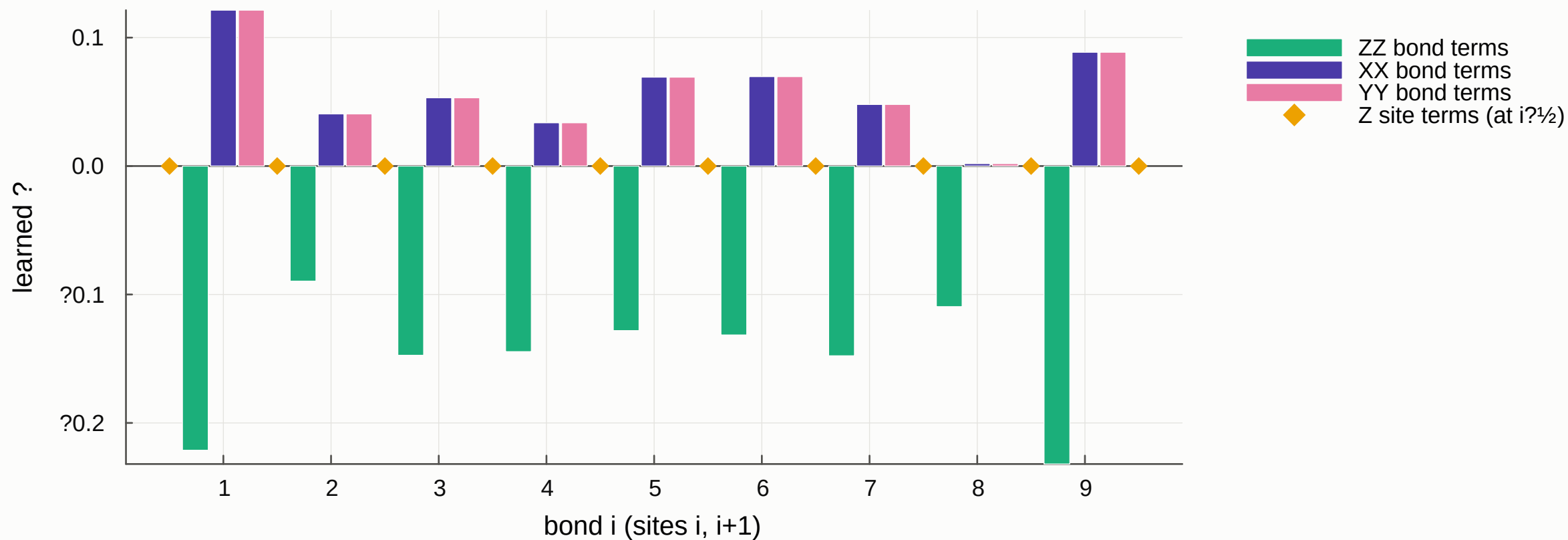
Alg 8 · squared loss (identity / bias coefficient -0.15)
