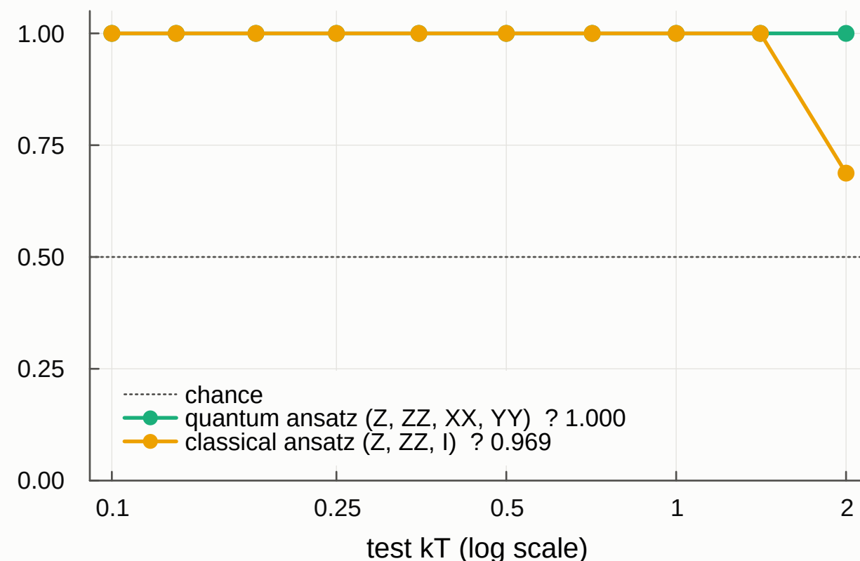
classical ansatz: score per test chain
