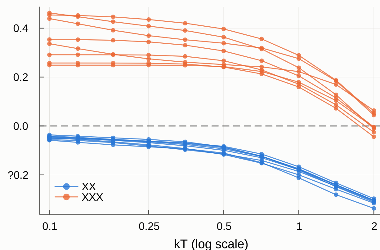
classical ansatz: score per test chain
