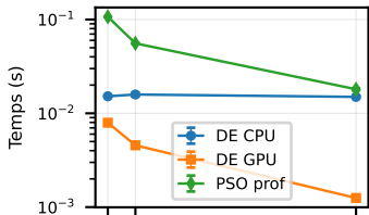
Rosenbrock, D=10
