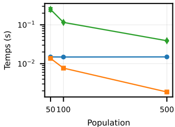
Rosenbrock, D=10
