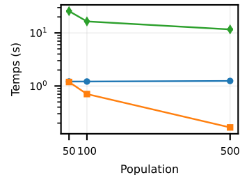
Rosenbrock, D=100
