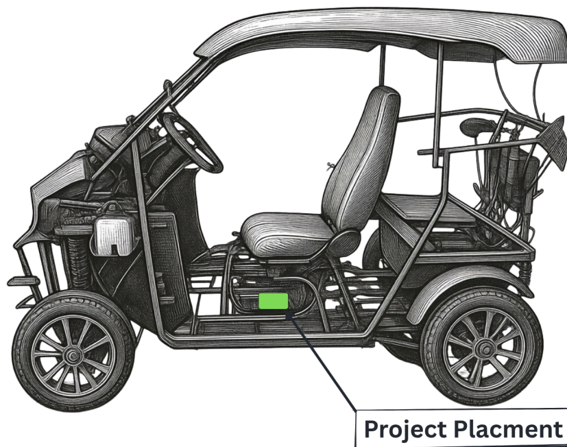
Figure 33: BAKO Motors vehicle with the ISS board installation location highlighted (green) — mounted beneath the driver seat adjacent to the MPPT controller, with short harness runs to the CAN bus, power rail, and sensor connectors.
