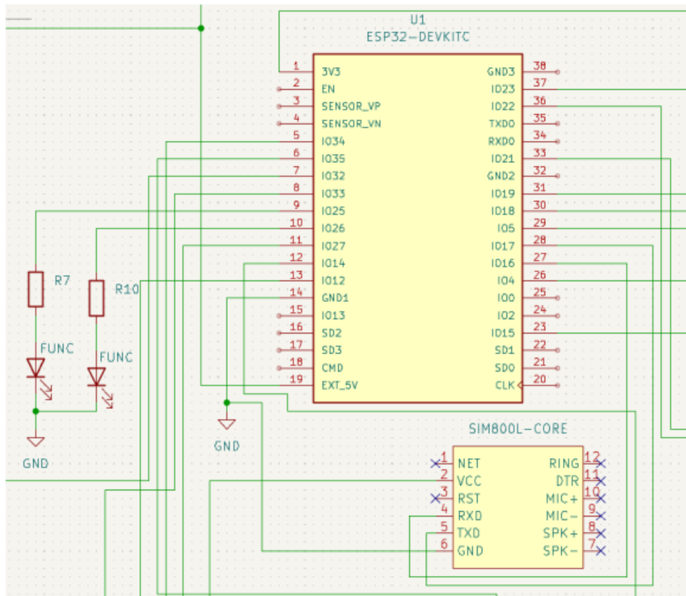
Figure: ESP32 +SIM800L Connections
