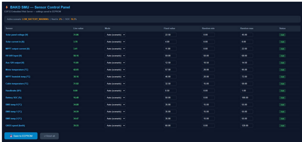
Figure 30: BAKO SMU Sensor Control Panel — browser-based interface served by the ESP32 firmware simulator, showing all 14 sensor channels with live values, scenario mode selectors, and manual override controls.
