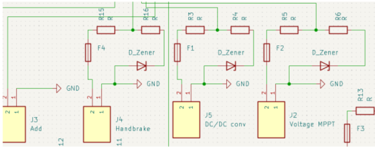
Figure: Voltage dividers
