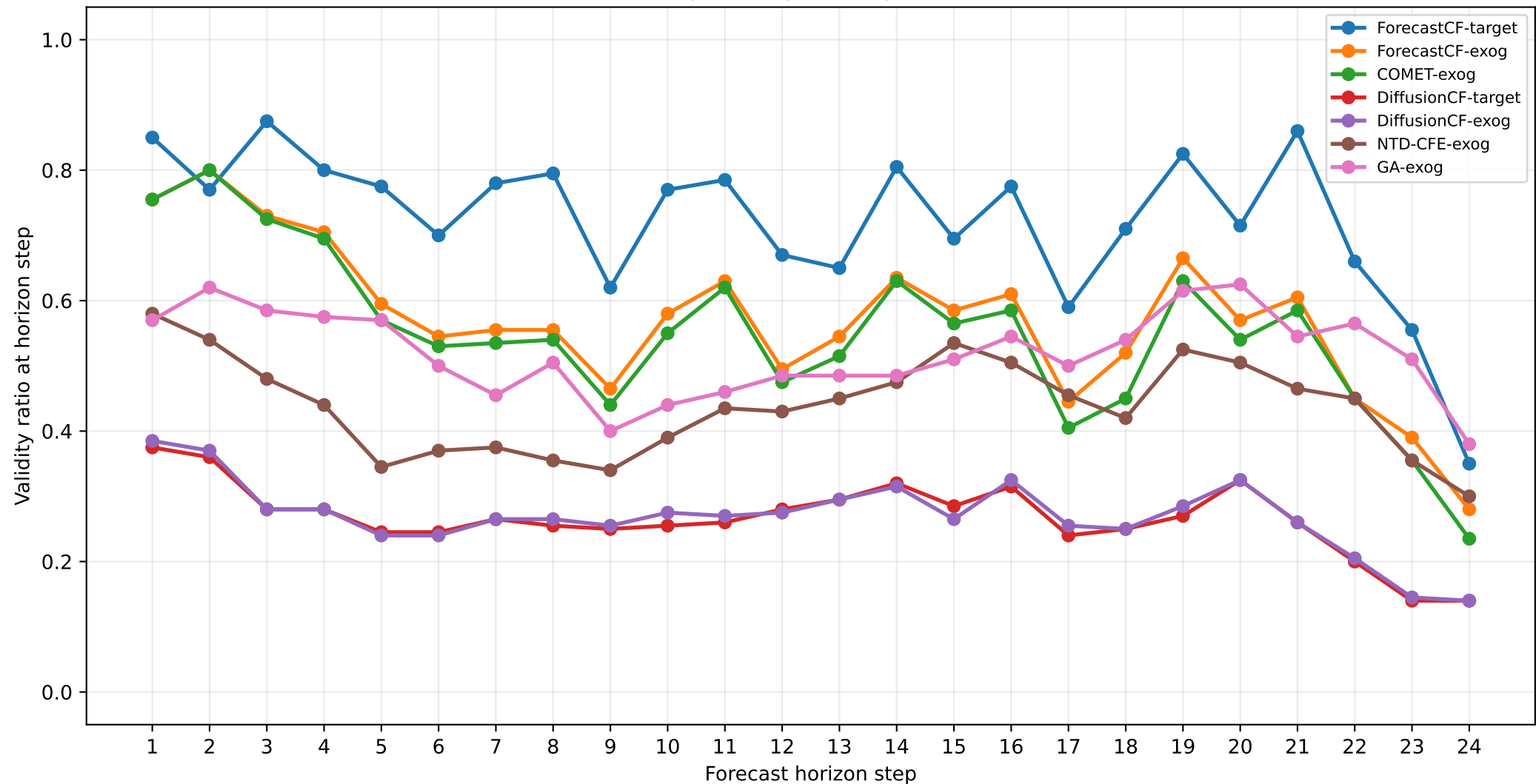
Per-horizon-step validity ratio by method — ETTh1
