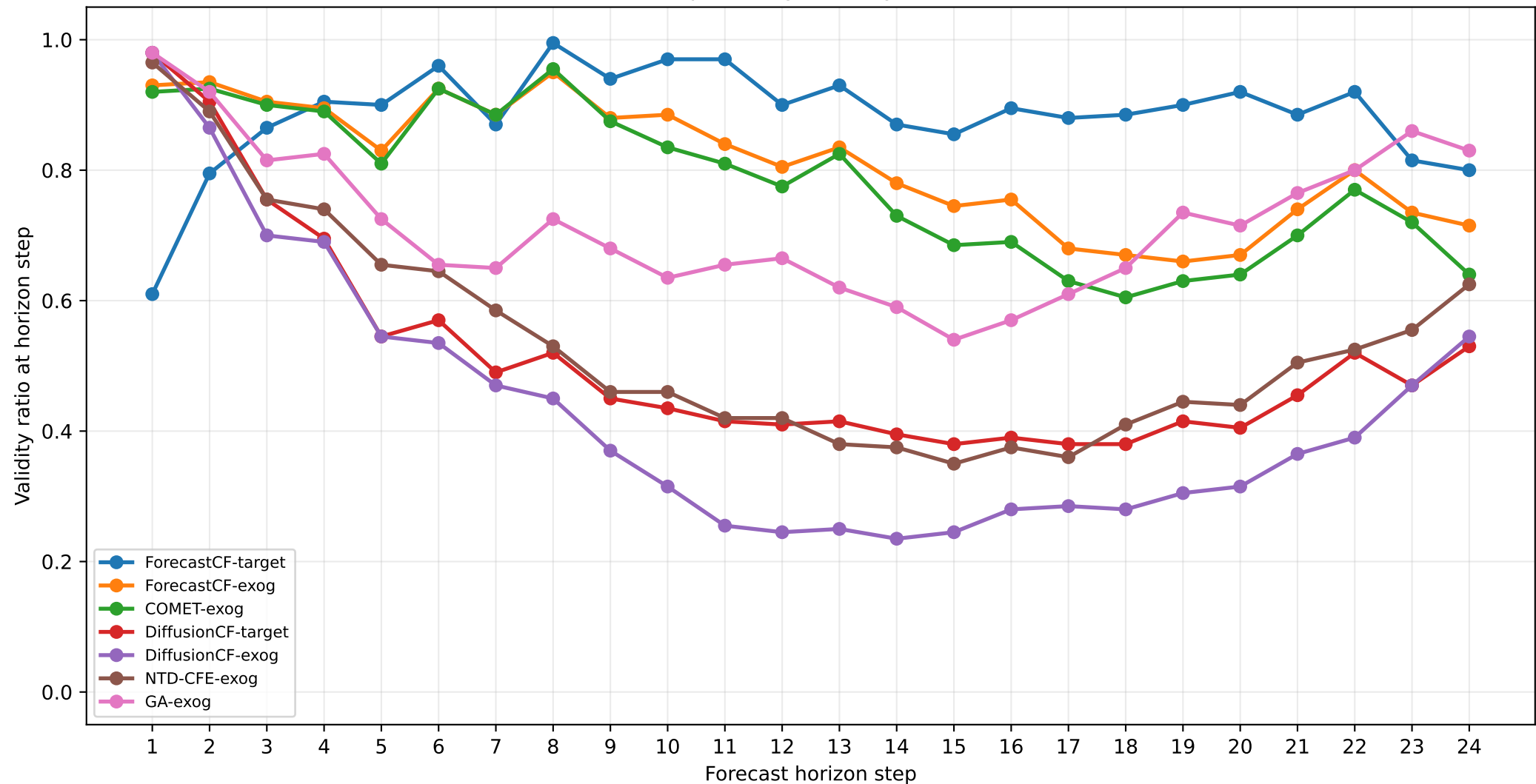
Per-horizon-step validity ratio by method — ETTh2
