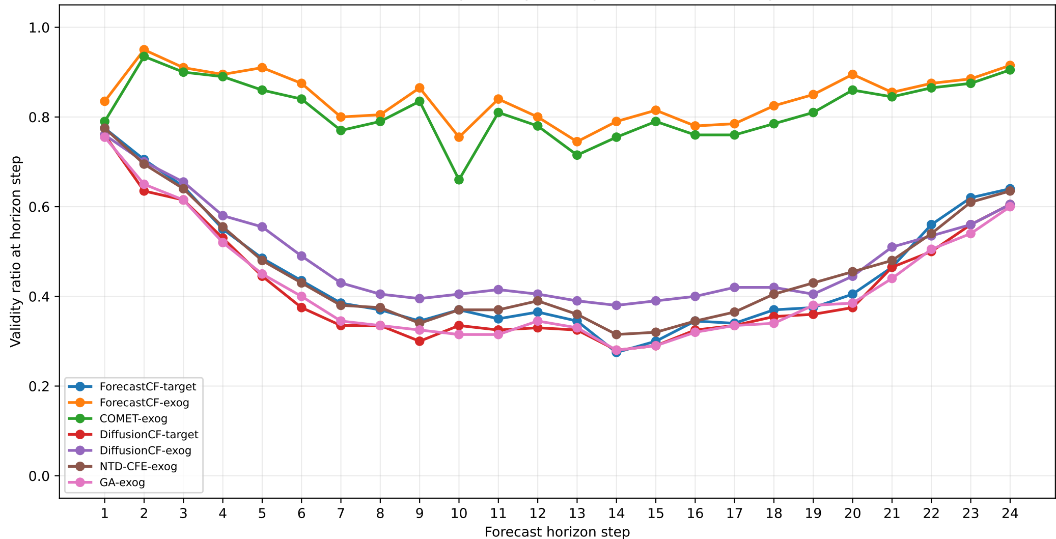
Per-horizon-step validity ratio by method — Electricity
