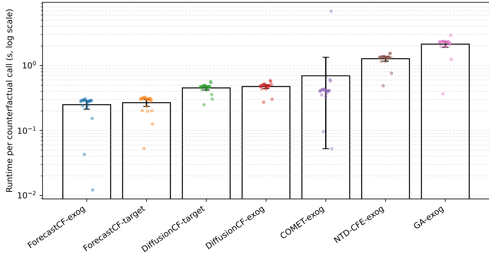
Counterfactual generation runtime across 21 datasets
