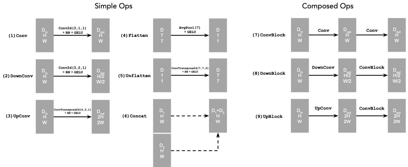
Figure 2: Standard UNet Operations
