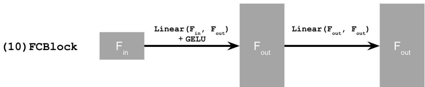
Figure 5: FCBlock for conditioning
