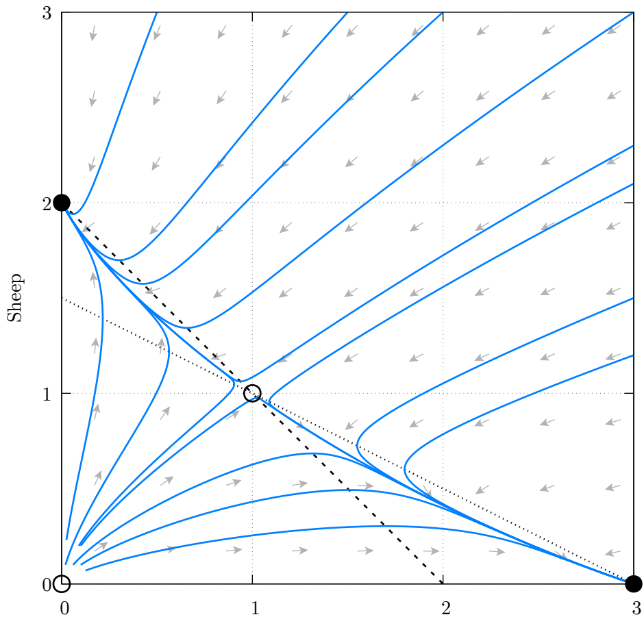
Phase Portrait (Rabbit and Sheep Model)
