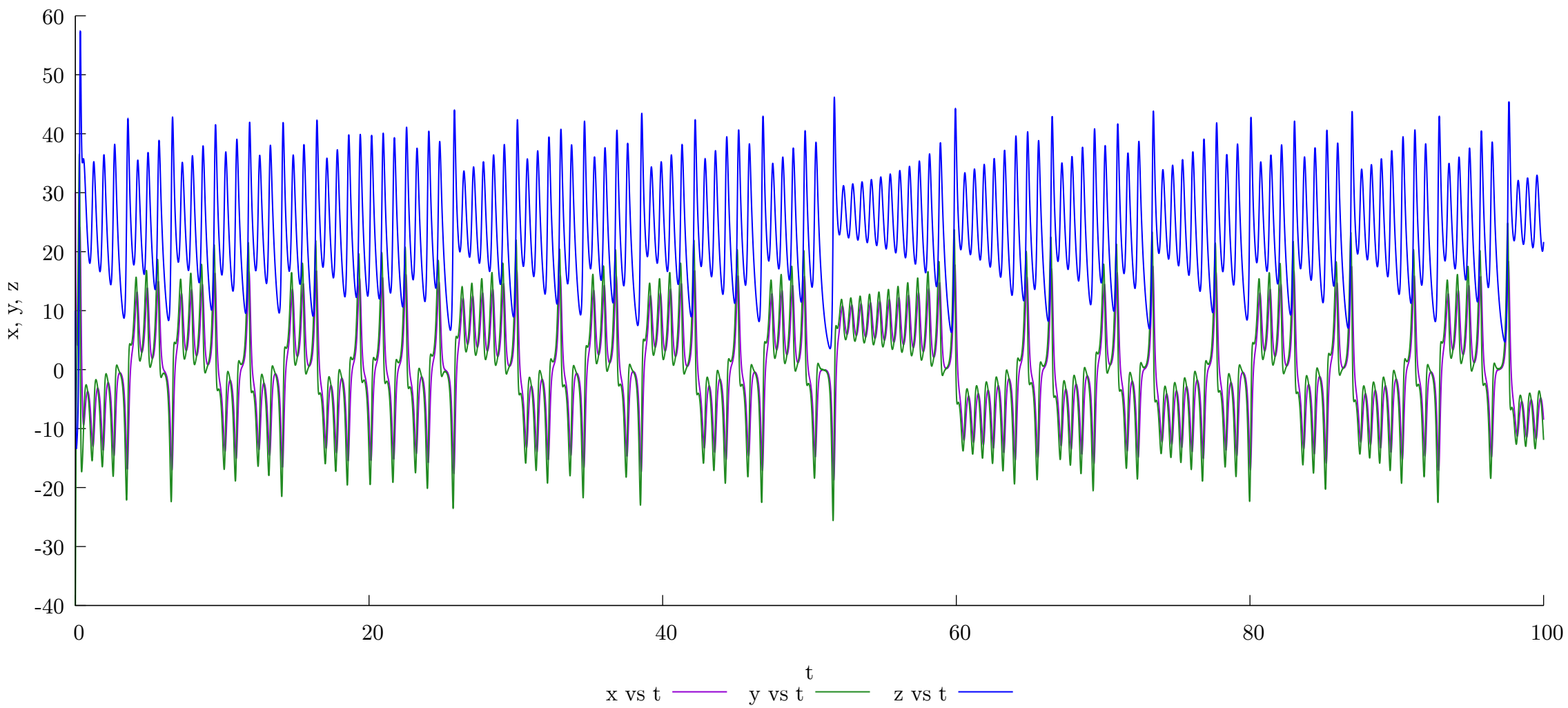
x, y and z vs t for initial condition (30, -40, 10)
