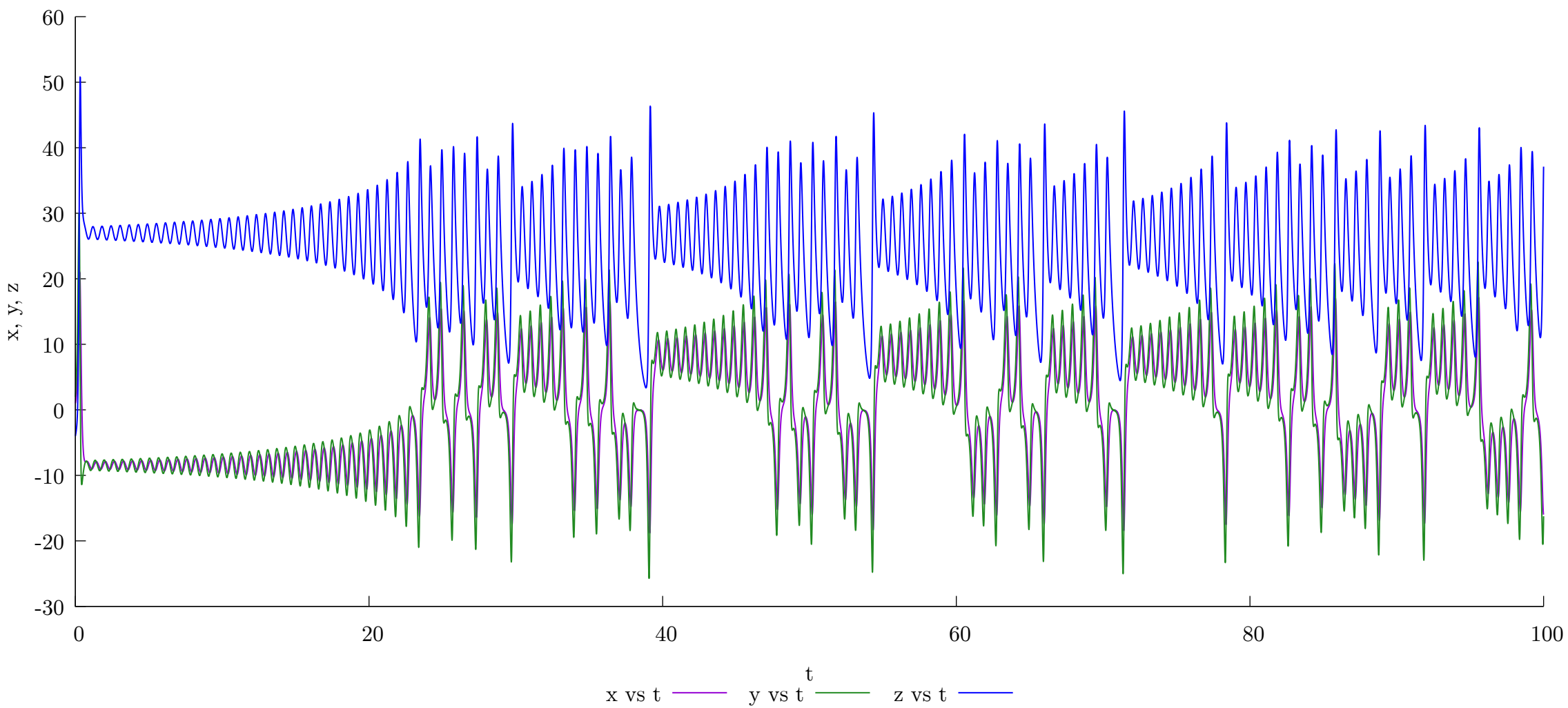
x, y and z vs t for initial condition (1, 2, -4)
