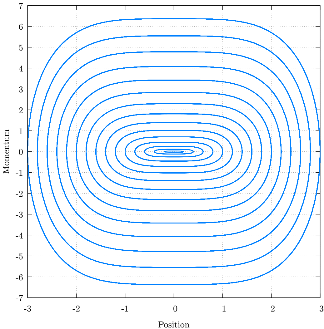
Phase Portrait (Pure Quartic Oscillator)
