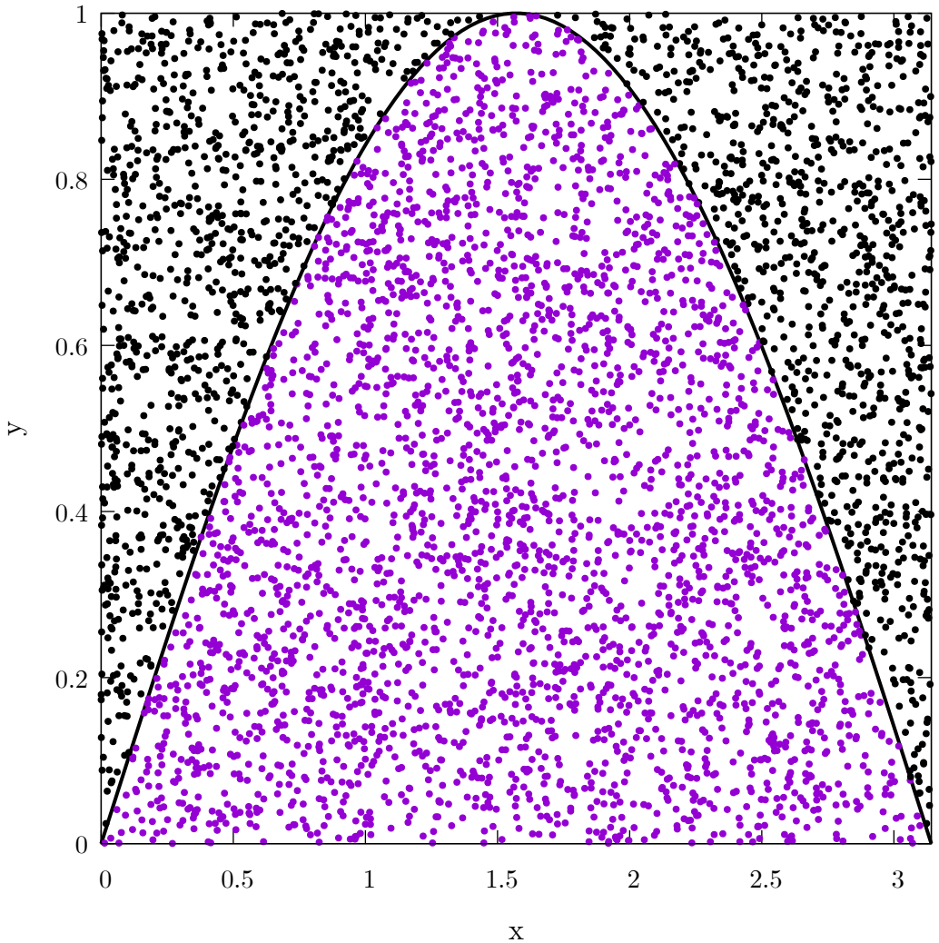
Monte Carlo Integral Estimation: Hit-or-Miss (N=5000)
