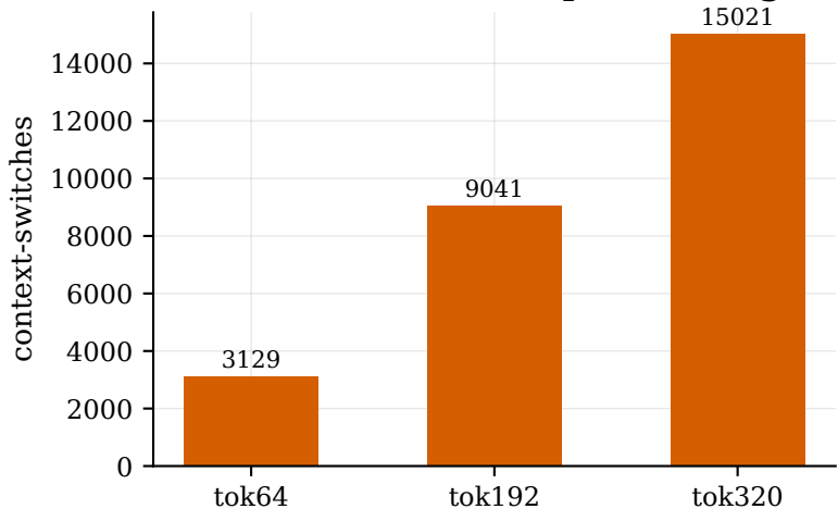
...but switches scale with output (waiting on GPU)
