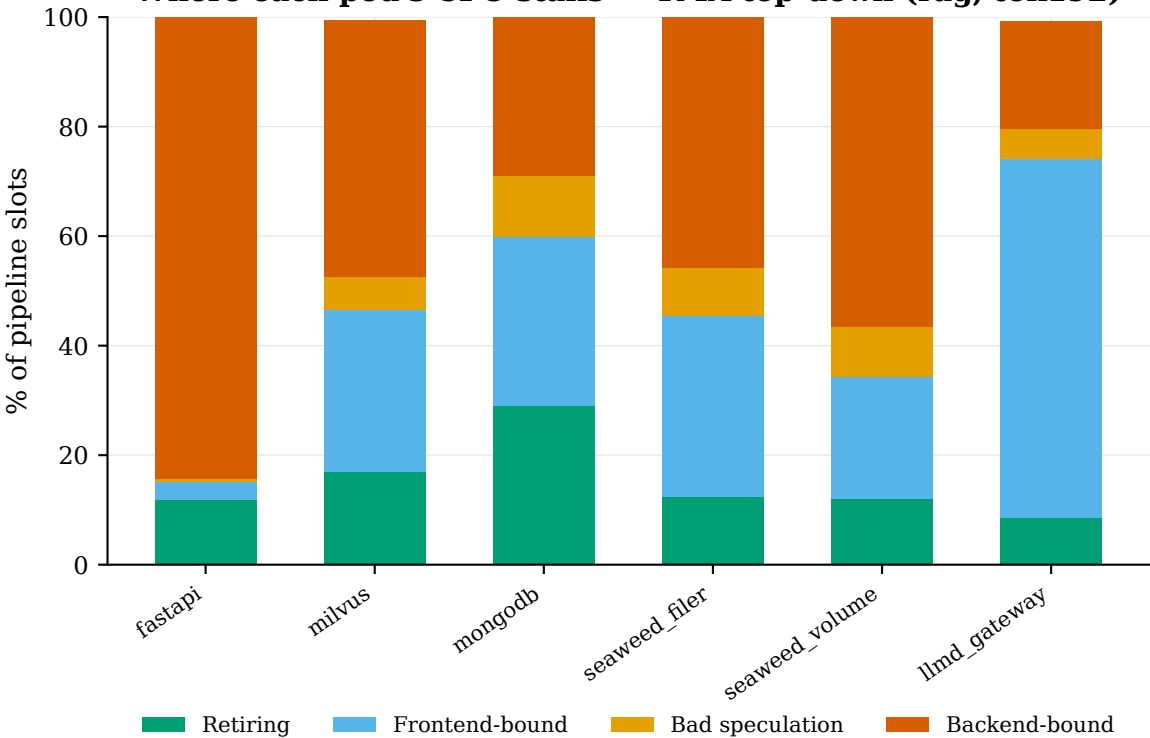
Where each pod's CPU stalls — TMA top-down (rag, tok192)
