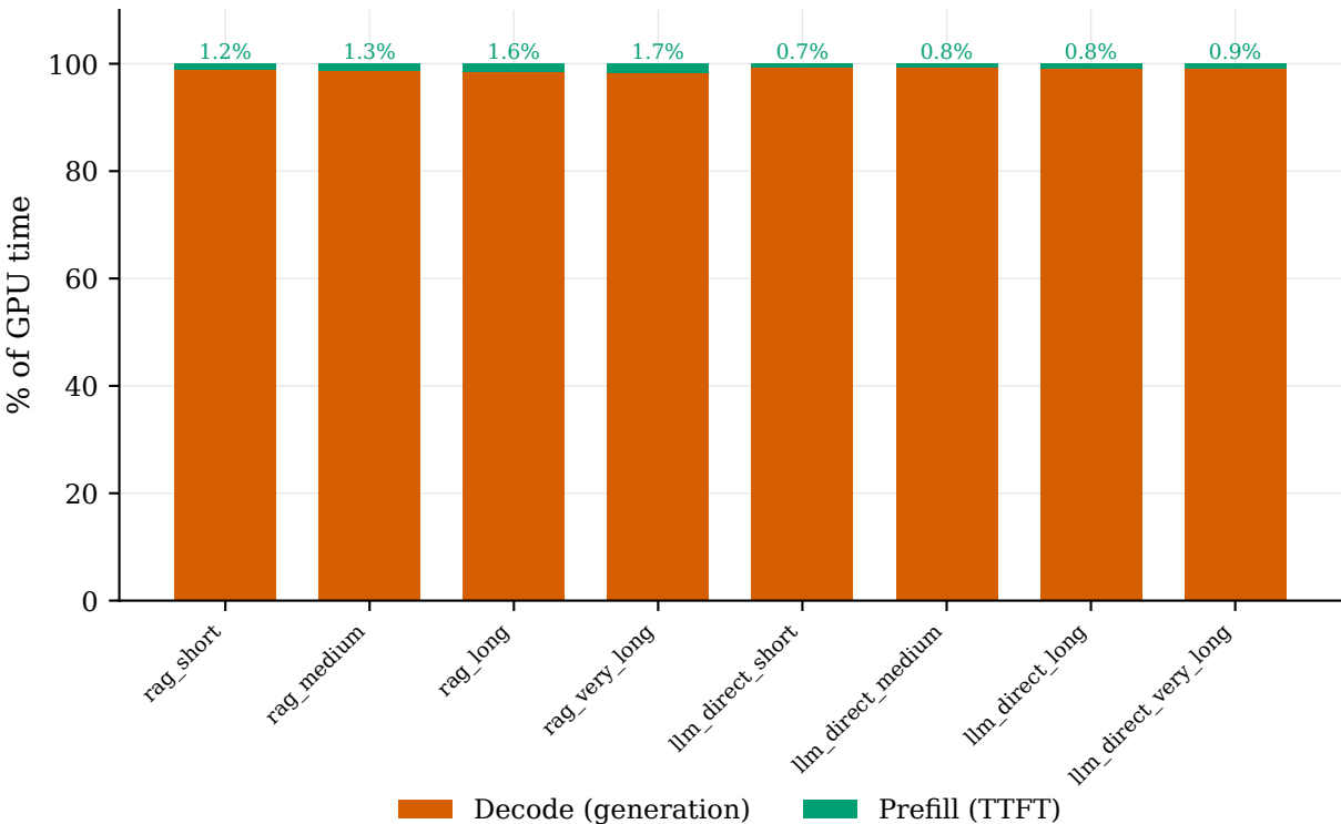
Prefill vs decode share of GPU time (tok320) — decode dominates
