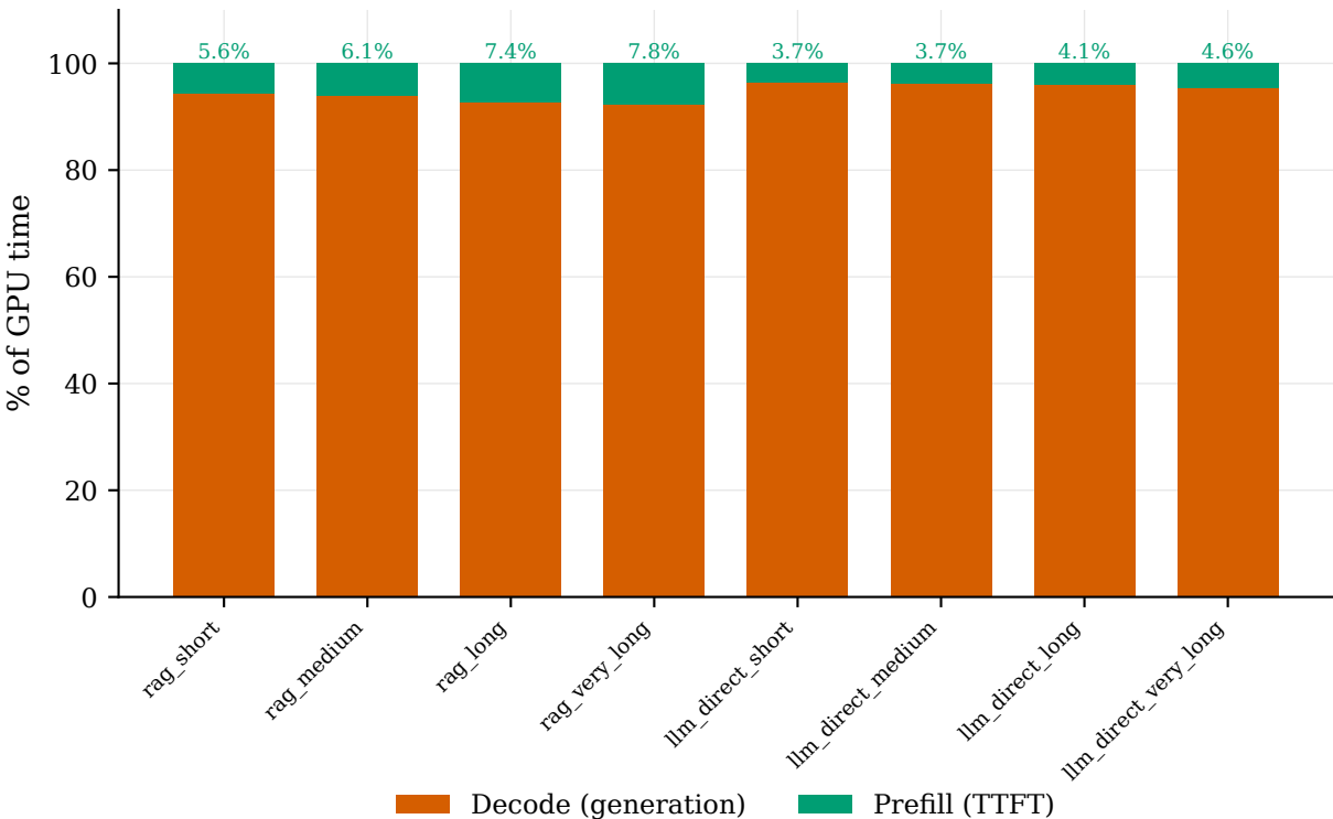
Prefill vs decode share of GPU time (tok64) — decode dominates
